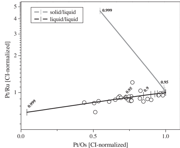
Fig. 9. A plot of batch extraction model calculations and ureilite data for Pt/Ru vs. Pt/Os (CI-chondrite normalized). Lines show model concentration ratios in residual solid (gray line) and residual C-rich liquid (heavy black line) after S-rich liquid extraction, with hash marks representing the fraction ( F ) of S-rich liquid removed from the system in increments of 0.05. Open circles are ureilite data from Rankenburg et al. (2008). Extraction of S-rich liquid from an immiscible liquid system seems to provide a good fit to the ureilite data.
